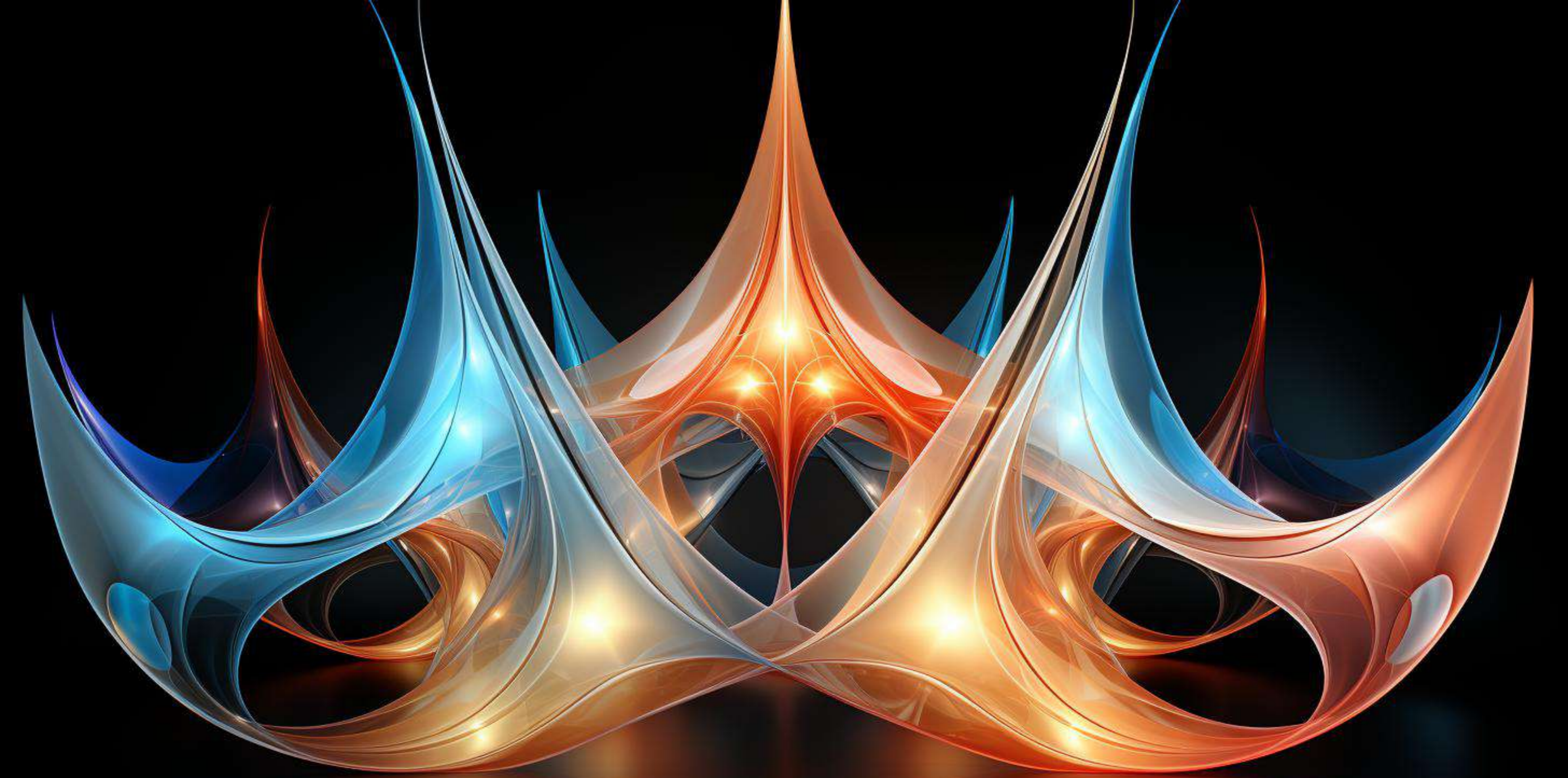
Binomial Expansion Fractal Geometry
