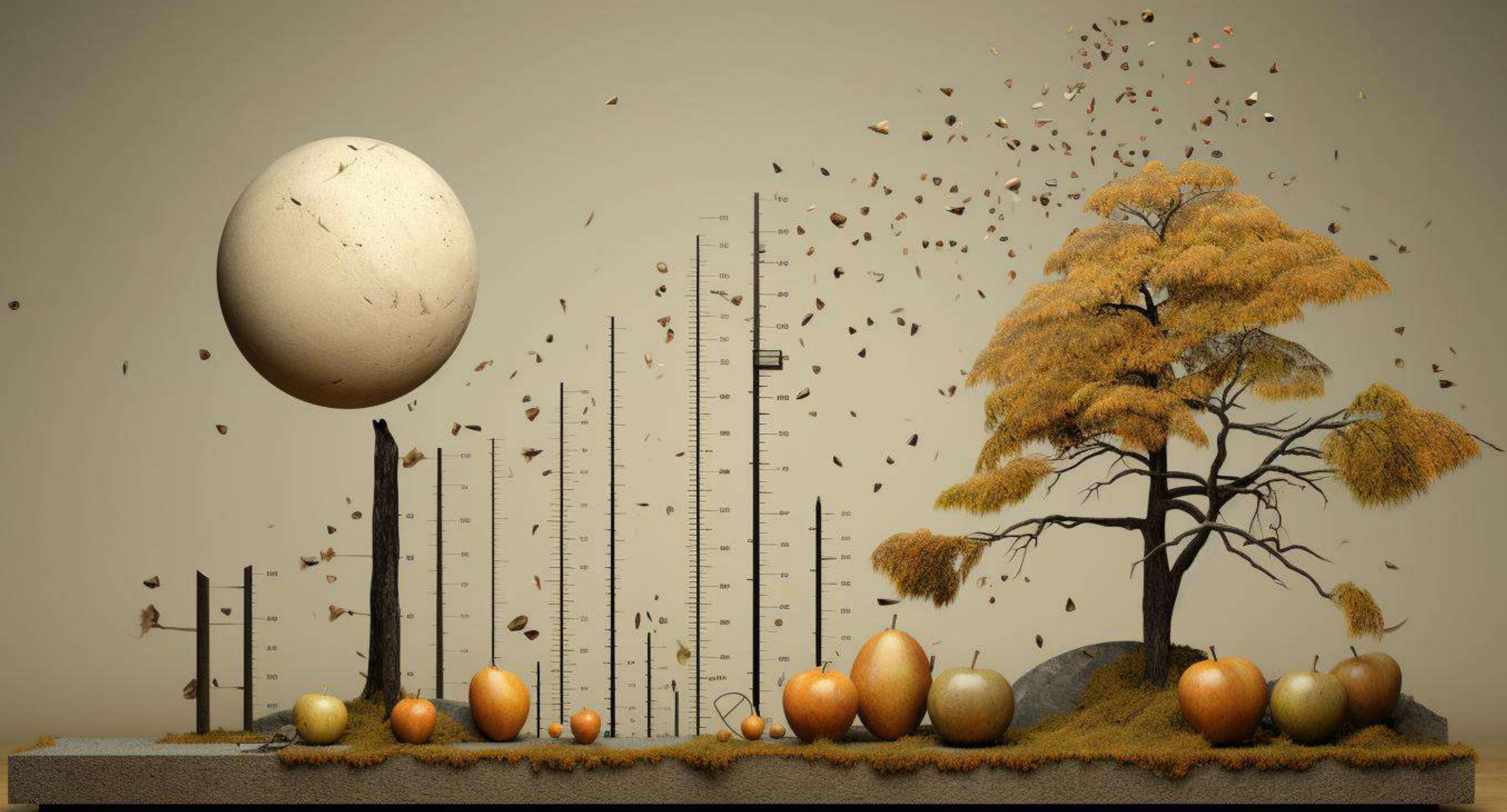
Natural Logarithm
